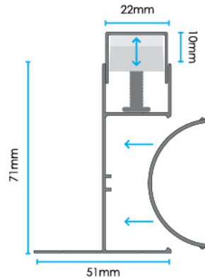
Top Profile, Adjustable Bar & DIY Nuts
